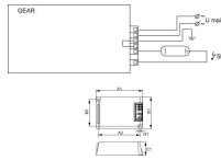
Scheda tecnica Philips HID-PV C 35 /S CDM 220-240V 50/60Hz
